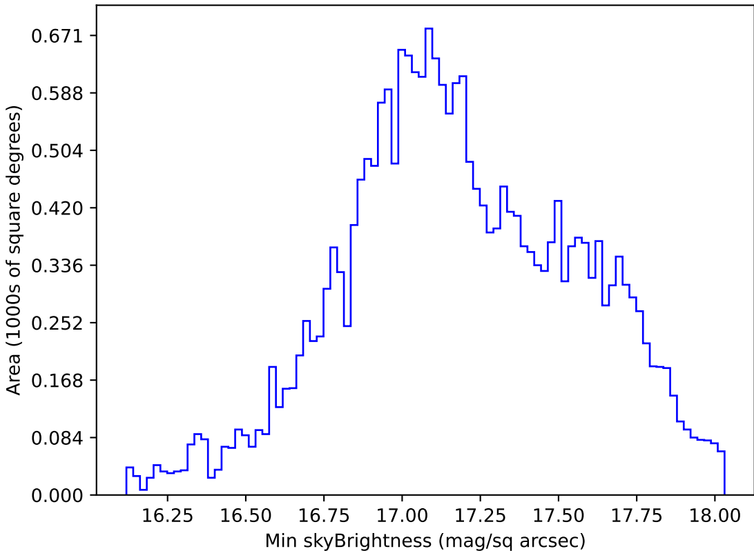
too_elab_r8_d3_giz_v3.4_10yrs All sky y band: Min skyBrightness
