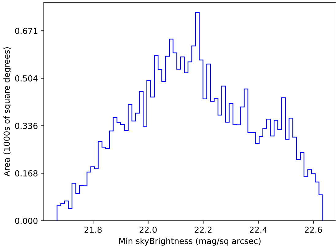
too_elab_r8_d3_giz_v3.4_10yrs All sky u band: Min skyBrightness
