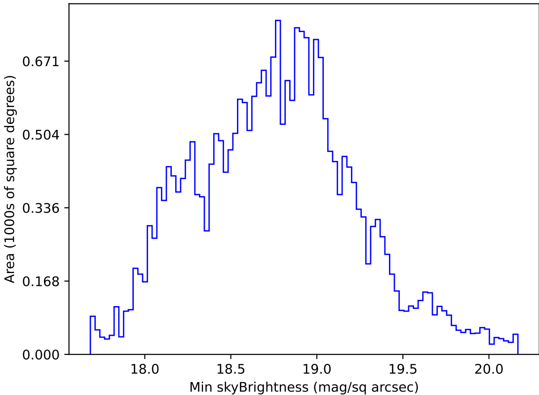
too_elab_r8_d3_giz_v3.4_10yrs All sky r band: Min skyBrightness
