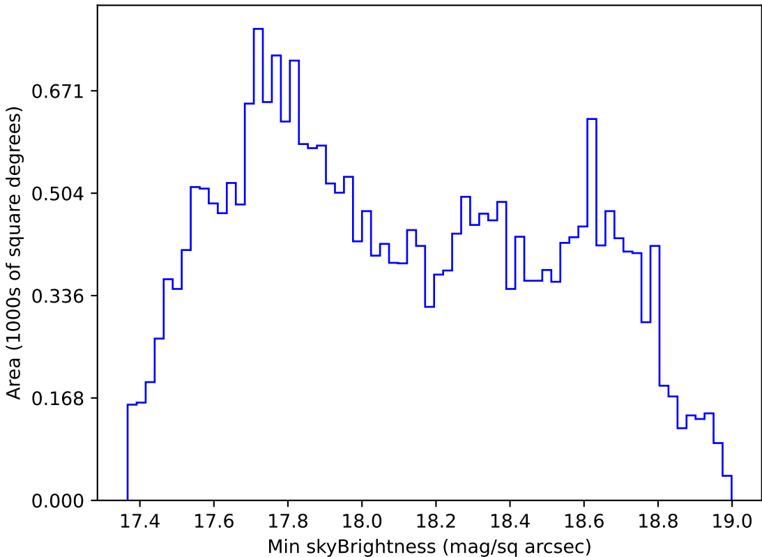
too_elab_r8_d3_giz_v3.4_10yrs All sky i band: Min skyBrightness
