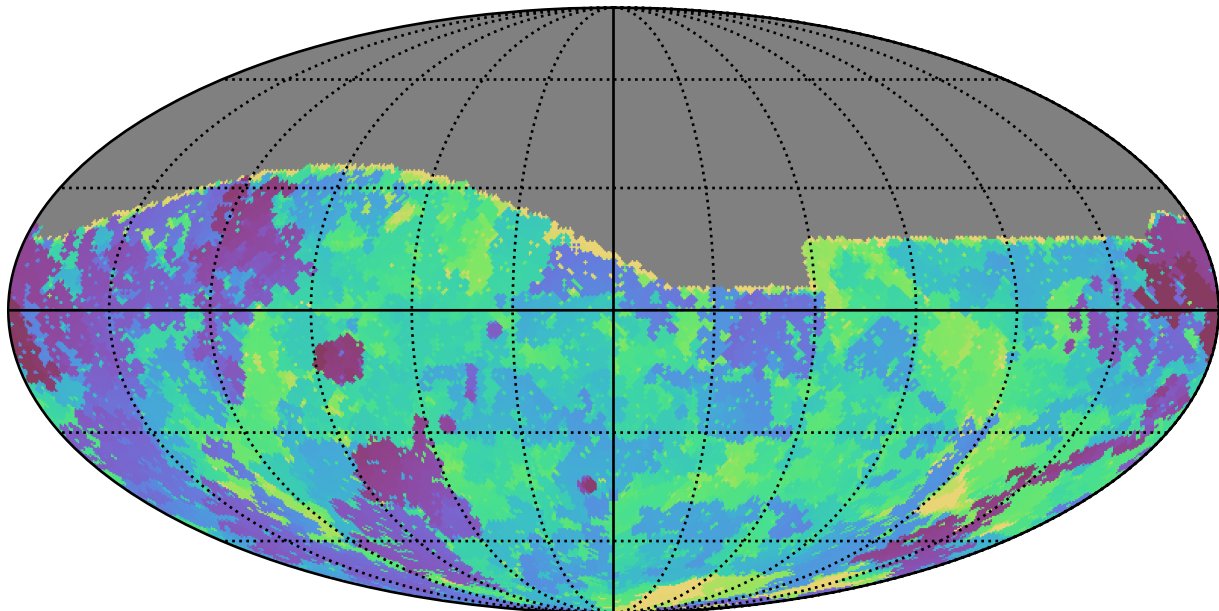
too_elab_r8_d3_giz_v3.4_10yrs All sky g band: Min skyBrightness
