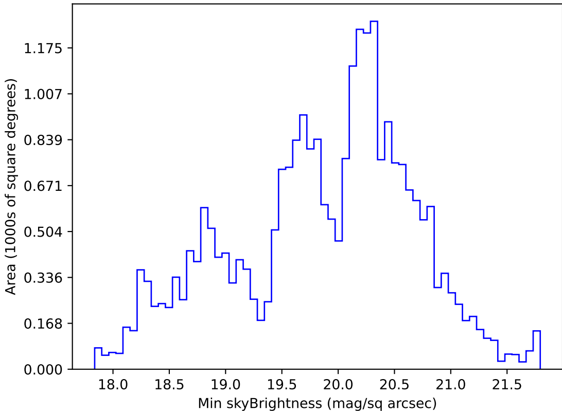
too_elab_r8_d3_giz_v3.4_10yrs All sky g band: Min skyBrightness
