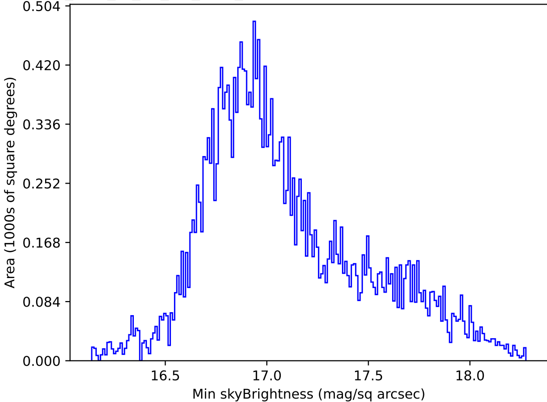
too_elab_r8_d3_giz_v3.4_10yrs All sky all bands: Min skyBrightness
