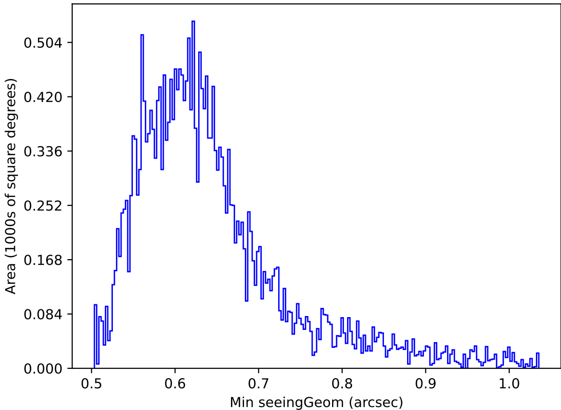
too_elab_r8_d3_giz_v3.4_10yrs Yr 1 z band: Min seeingGeom
