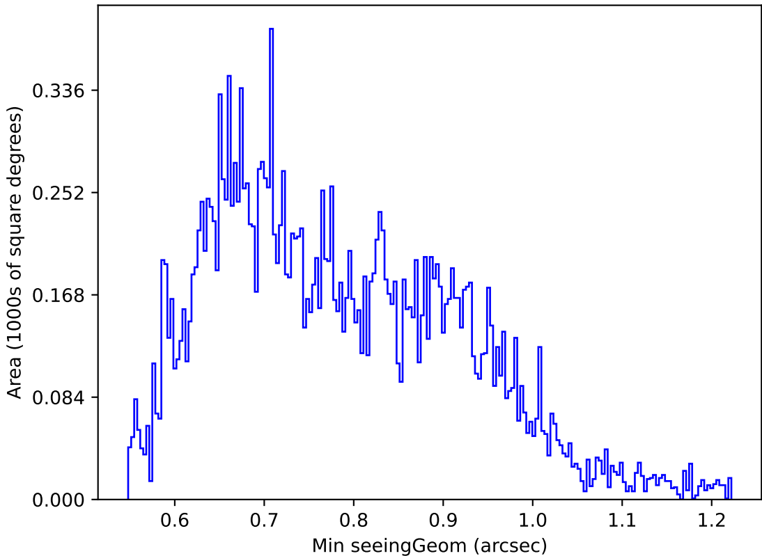
too_elab_r8_d3_giz_v3.4_10yrs Yr 1 u band: Min seeingGeom
