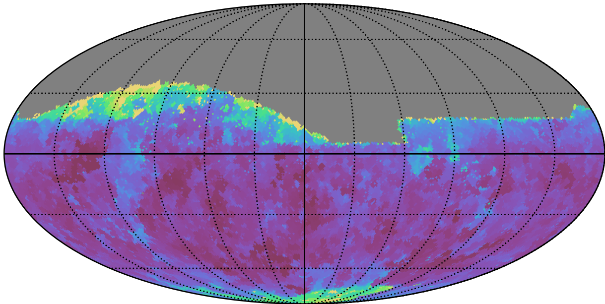
too_elab_r8_d3_giz_v3.4_10yrs Yr 1 i band: Min seeingGeom
