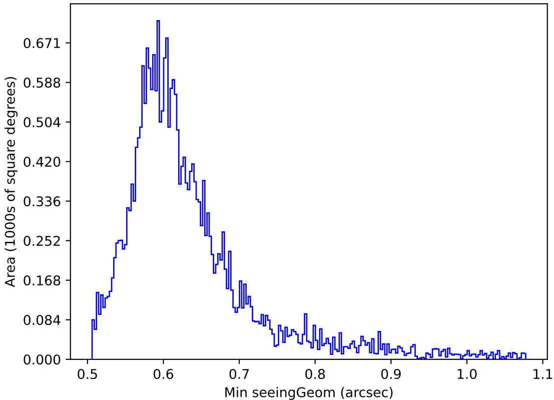
too_elab_r8_d3_giz_v3.4_10yrs Yr 1 i band: Min seeingGeom
