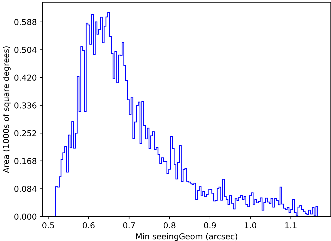
too_elab_r8_d3_giz_v3.4_10yrs Yr 1 g band: Min seeingGeom
