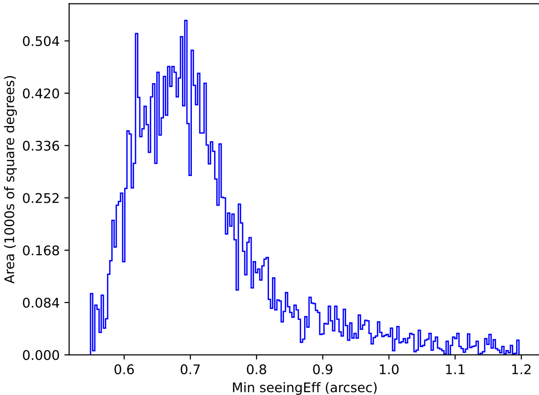
too_elab_r8_d3_giz_v3.4_10yrs Yr 1 z band: Min seeingEff
