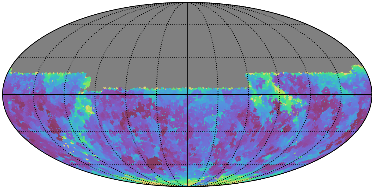
too_elab_r8_d3_giz_v3.4_10yrs Yr 1 y band: Min seeingEff
