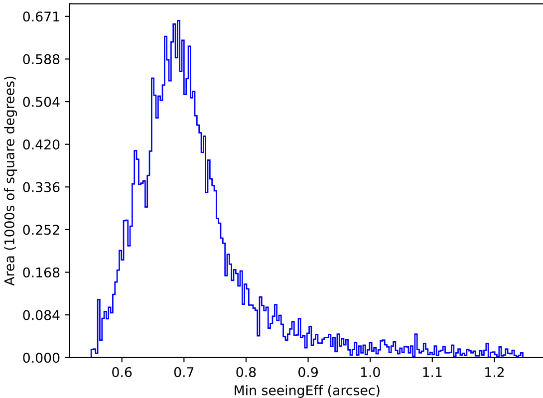
too_elab_r8_d3_giz_v3.4_10yrs Yr 1 r band: Min seeingEff
