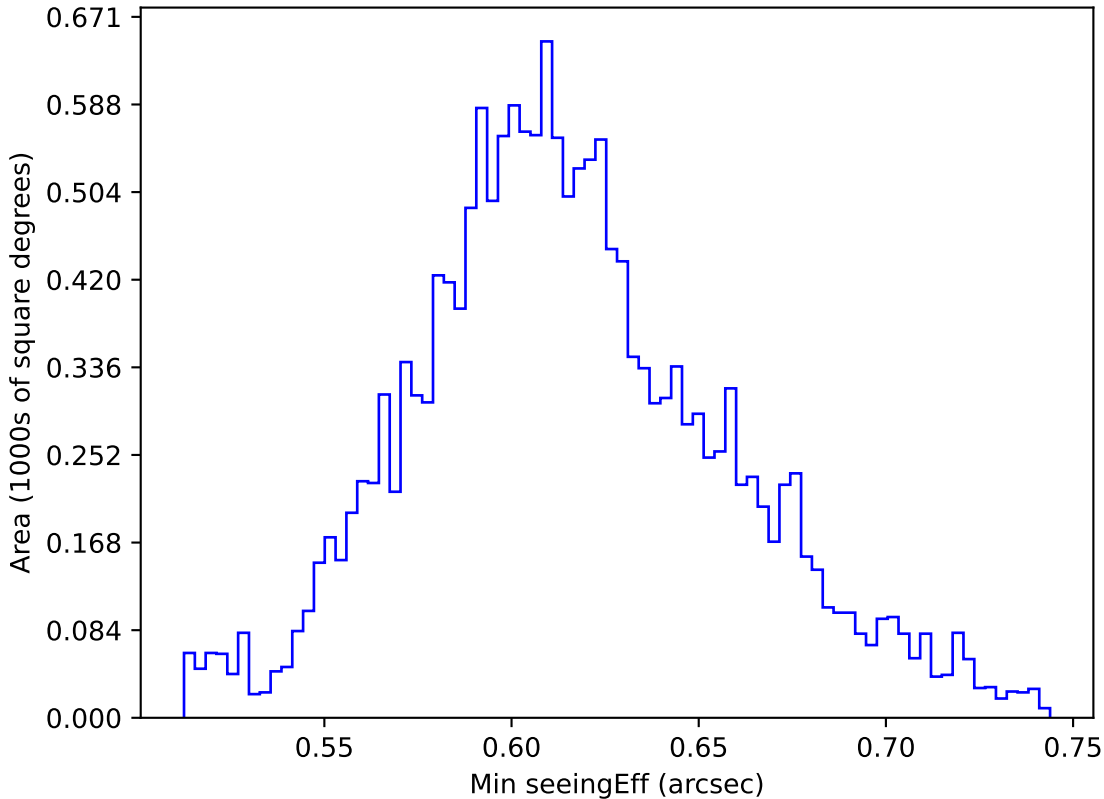
too_elab_r8_d3_giz_v3.4_10yrs WFD z band: Min seeingEff
