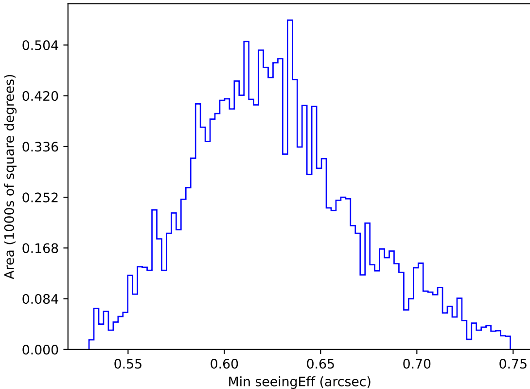
too_elab_r8_d3_giz_v3.4_10yrs WFD y band: Min seeingEff
