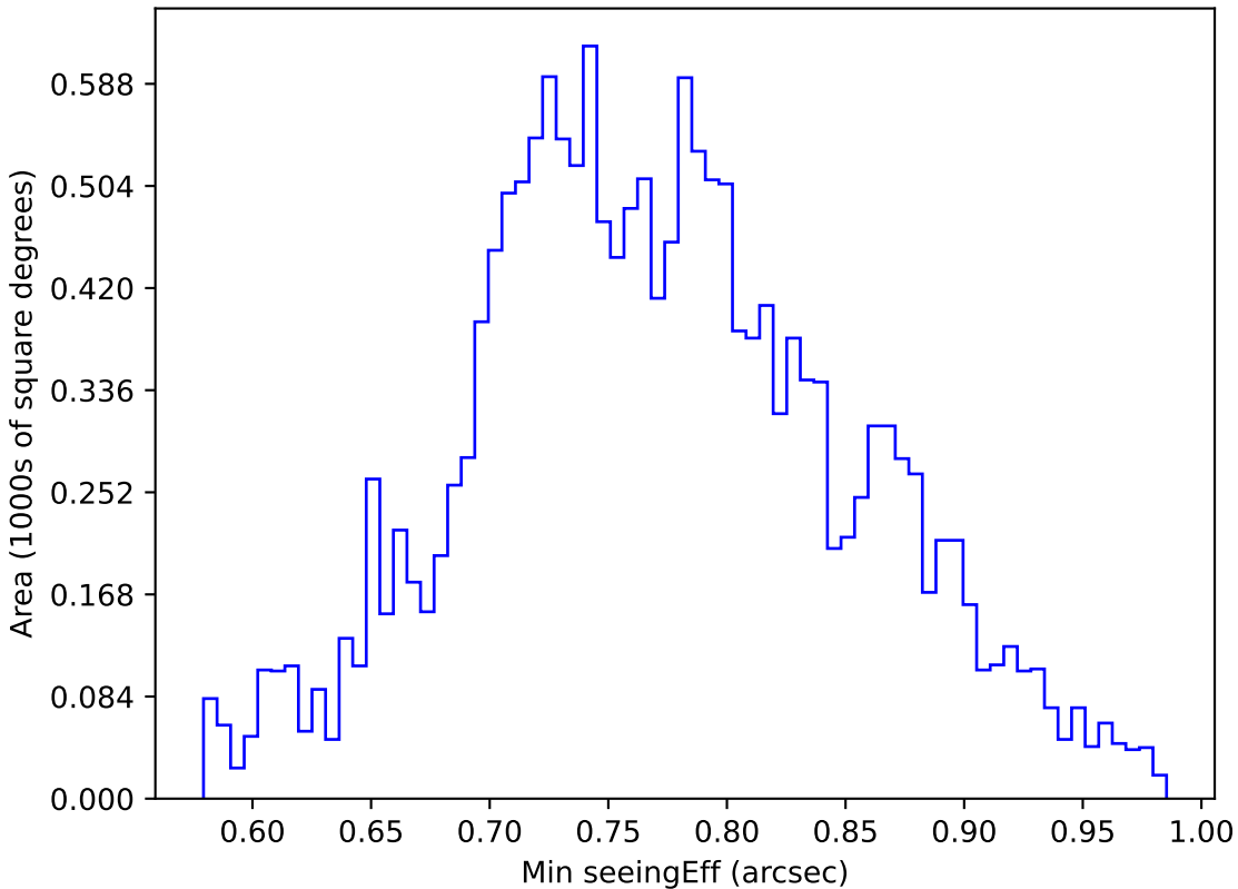
too_elab_r8_d3_giz_v3.4_10yrs WFD u band: Min seeingEff
