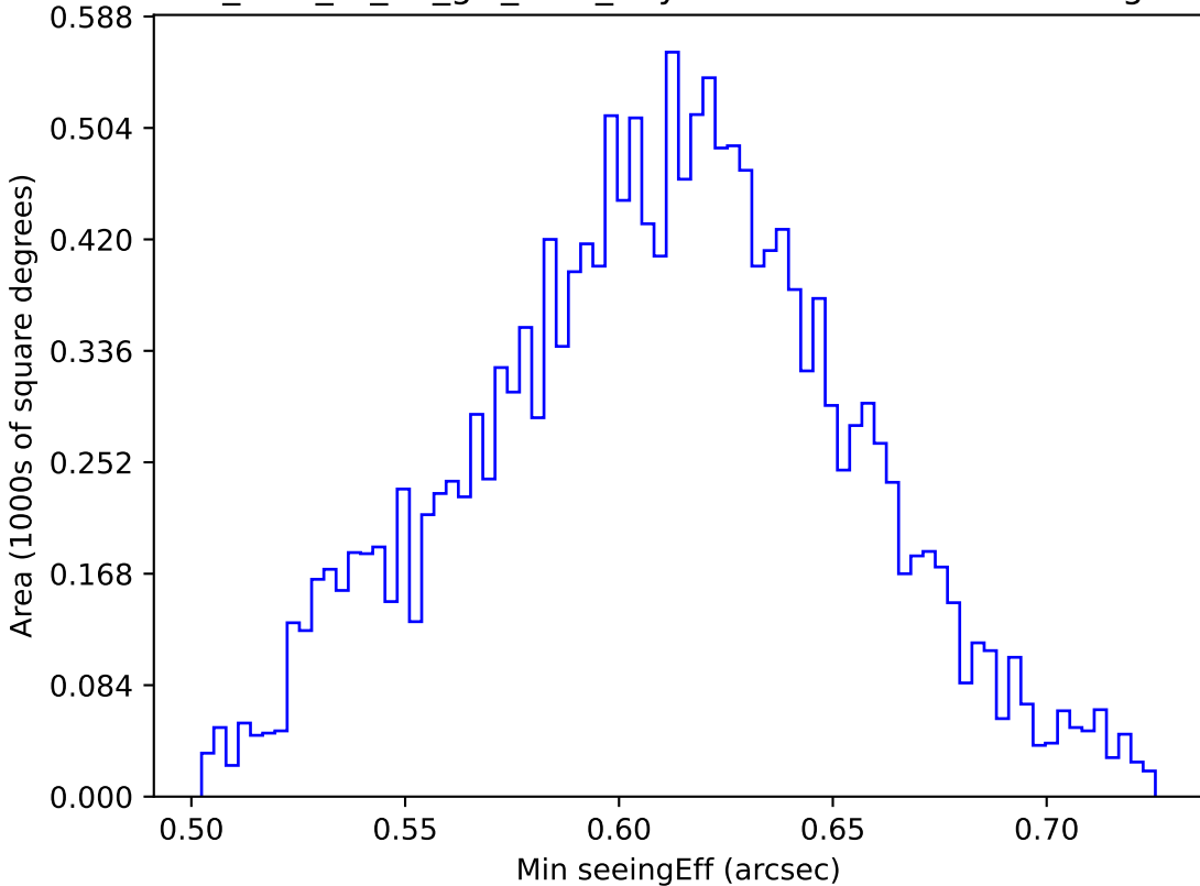
too_elab_r8_d3_giz_v3.4_10yrs WFD r band: Min seeingEff
