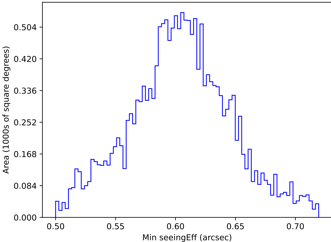
too_elab_r8_d3_giz_v3.4_10yrs WFD i band: Min seeingEff
