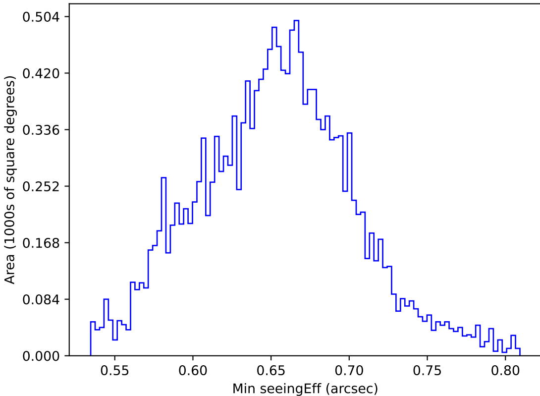
too_elab_r8_d3_giz_v3.4_10yrs WFD g band: Min seeingEff
