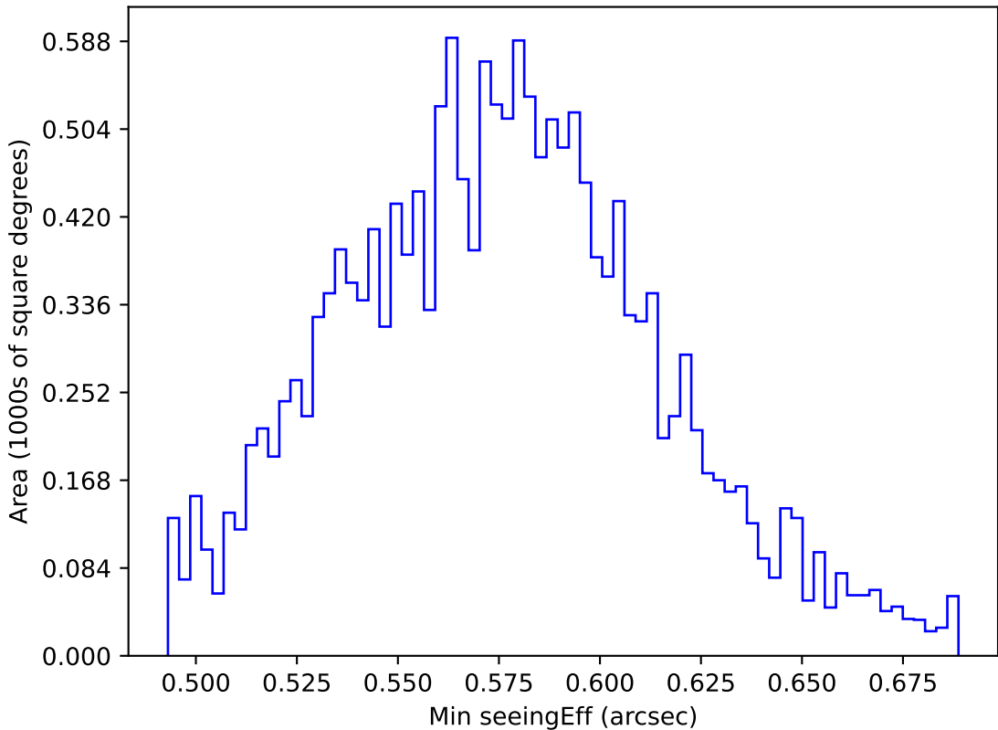
too_elab_r8_d3_giz_v3.4_10yrs WFD all bands: Min seeingEff
