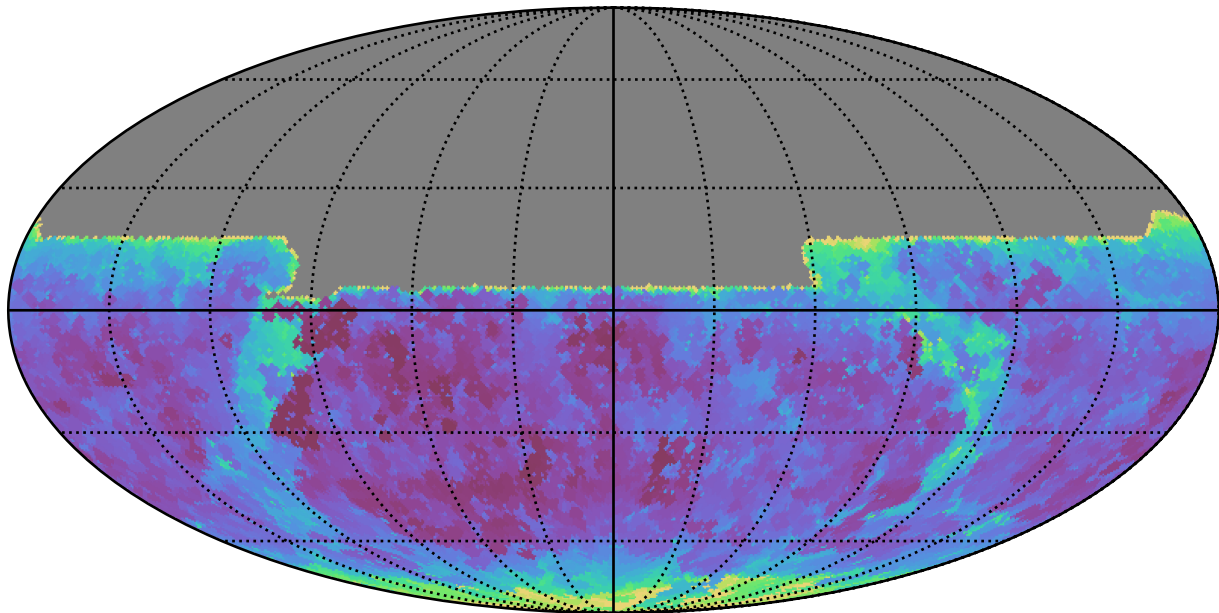
too_elab_r8_d3_giz_v3.4_10yrs All sky y band: Min seeingEff
