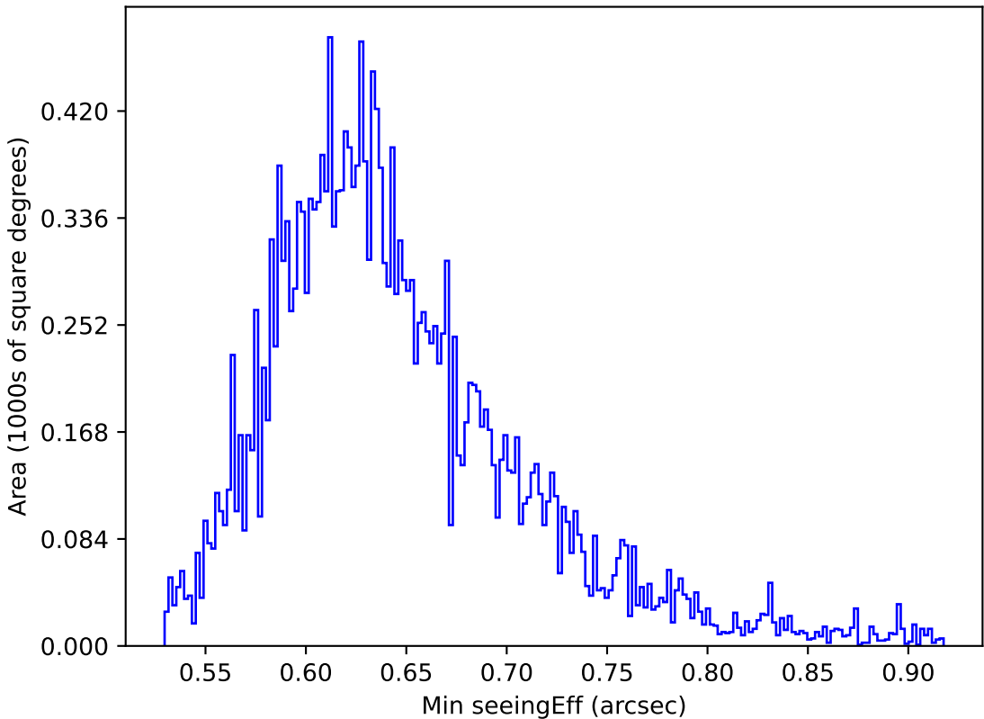
too_elab_r8_d3_giz_v3.4_10yrs All sky y band: Min seeingEff
