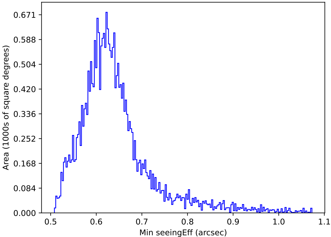
too_elab_r8_d3_giz_v3.4_10yrs All sky r band: Min seeingEff
