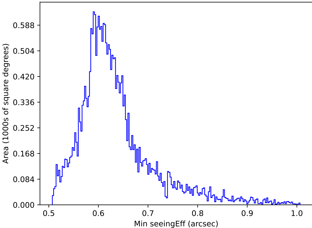
too_elab_r8_d3_giz_v3.4_10yrs All sky i band: Min seeingEff
