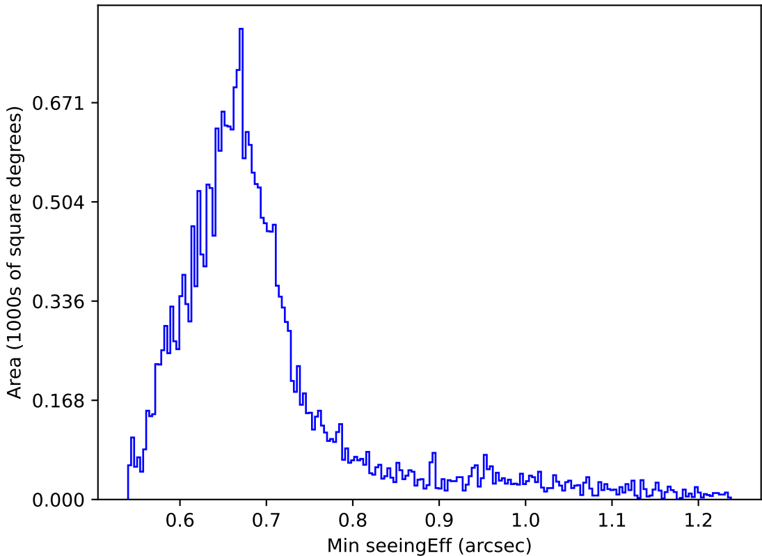
too_elab_r8_d3_giz_v3.4_10yrs All sky g band: Min seeingEff
