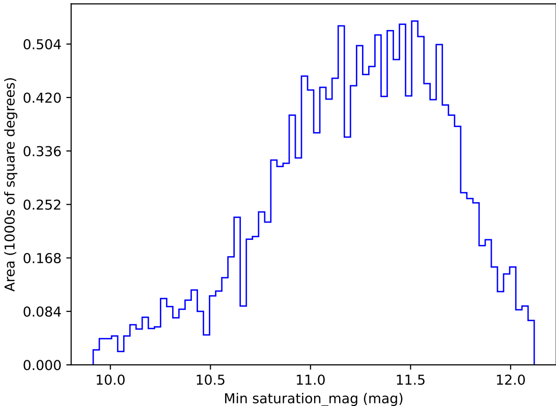
too_elab_r8_d3_giz_v3.4_10yrs WFD y band: Min saturation_mag
