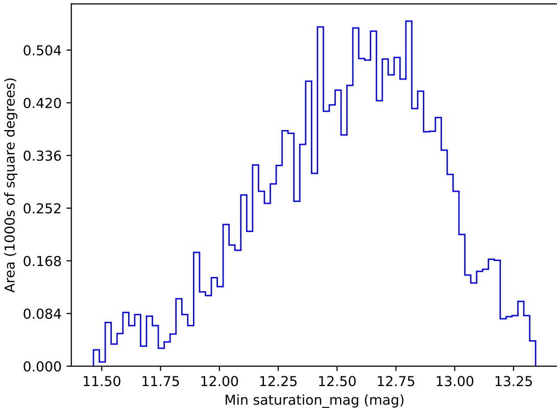
too_elab_r8_d3_giz_v3.4_10yrs WFD r band: Min saturation_mag
