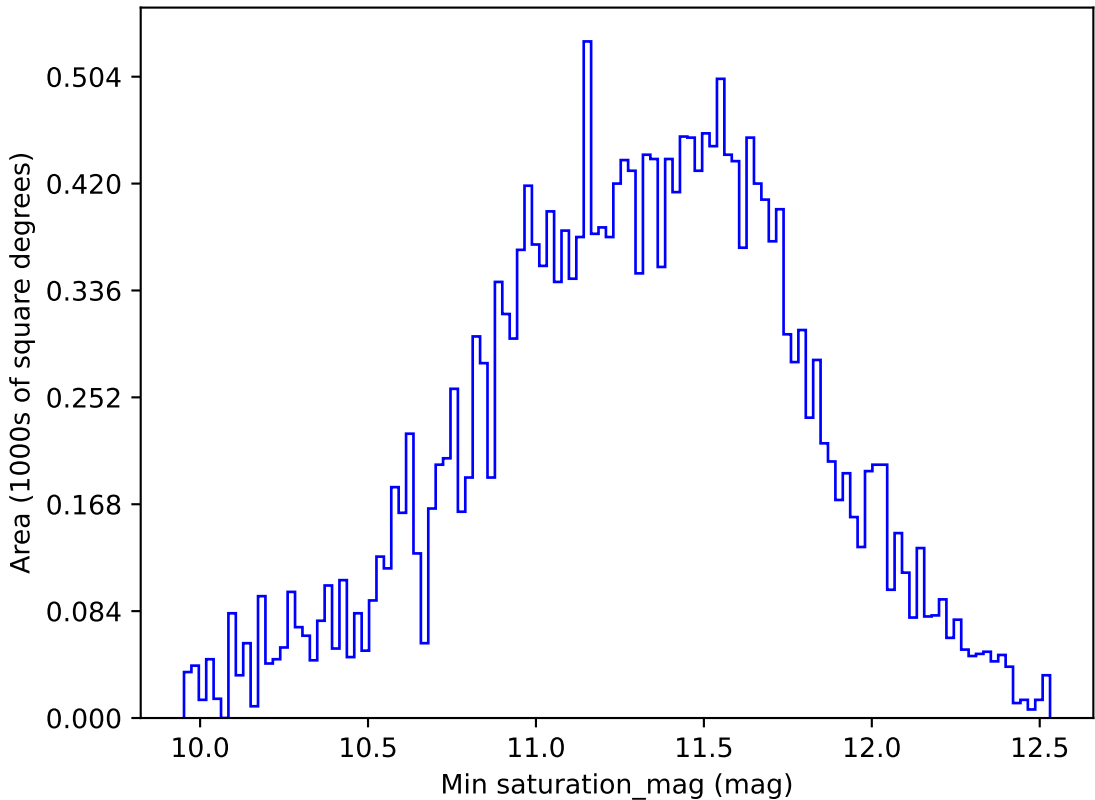
too_elab_r8_d3_giz_v3.4_10yrs All sky y band: Min saturation_mag
