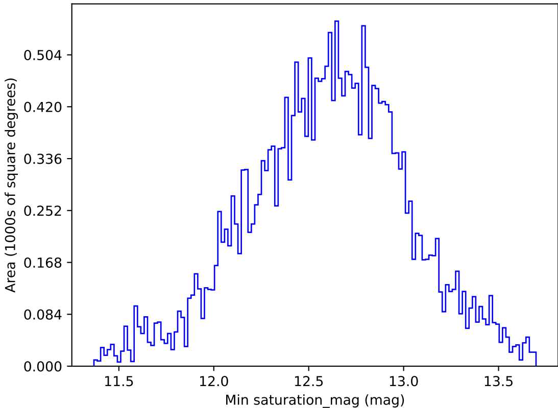
too_elab_r8_d3_giz_v3.4_10yrs All sky r band: Min saturation_mag
