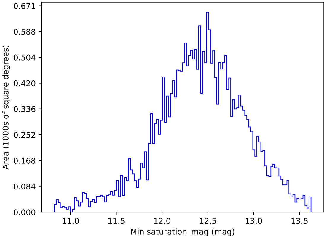
too_elab_r8_d3_giz_v3.4_10yrs All sky i band: Min saturation_mag
