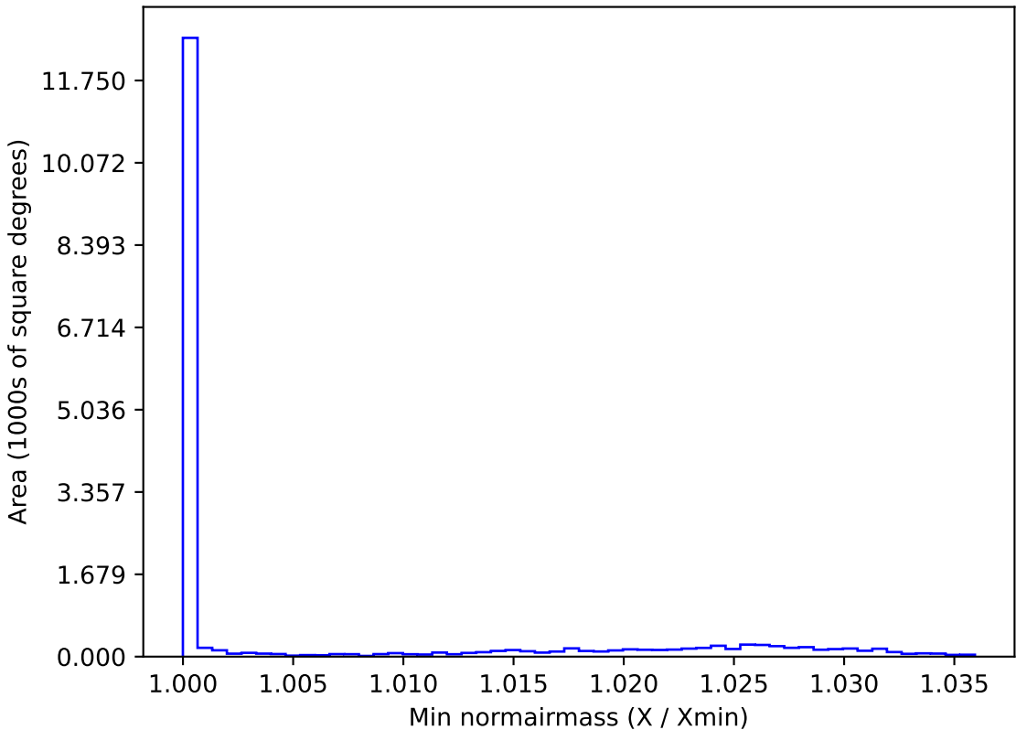
too_elab_r8_d3_giz_v3.4_10yrs WFD z band: Min normairmass
