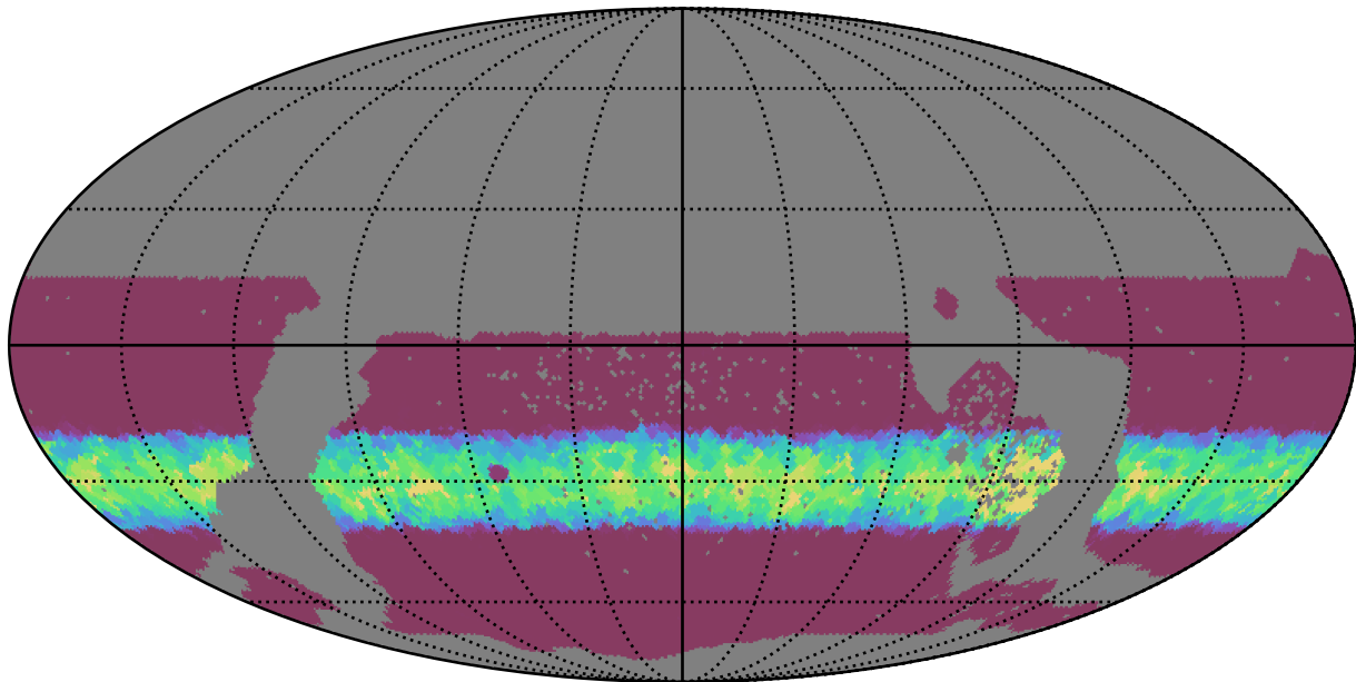
too_elab_r8_d3_giz_v3.4_10yrs WFD y band: Min normairmass
