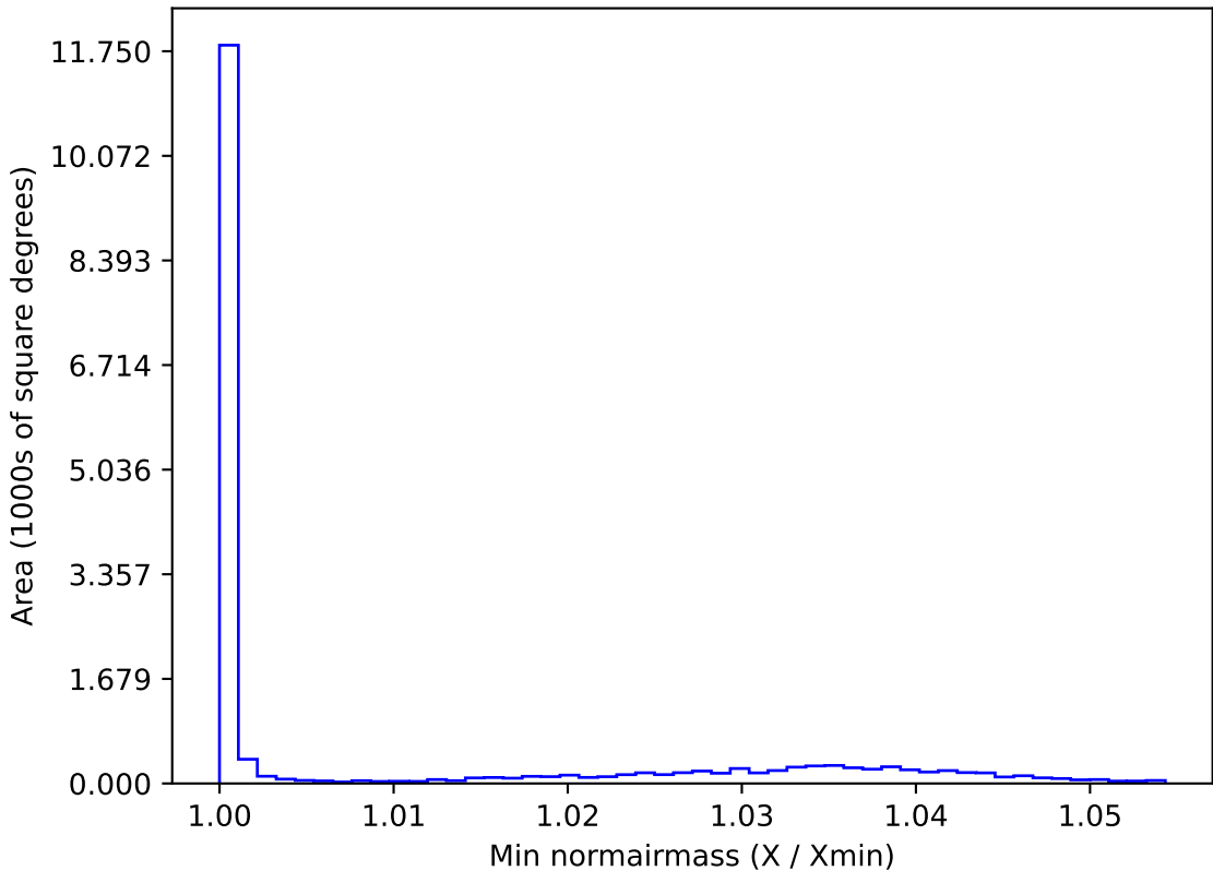
too_elab_r8_d3_giz_v3.4_10yrs WFD u band: Min normairmass
