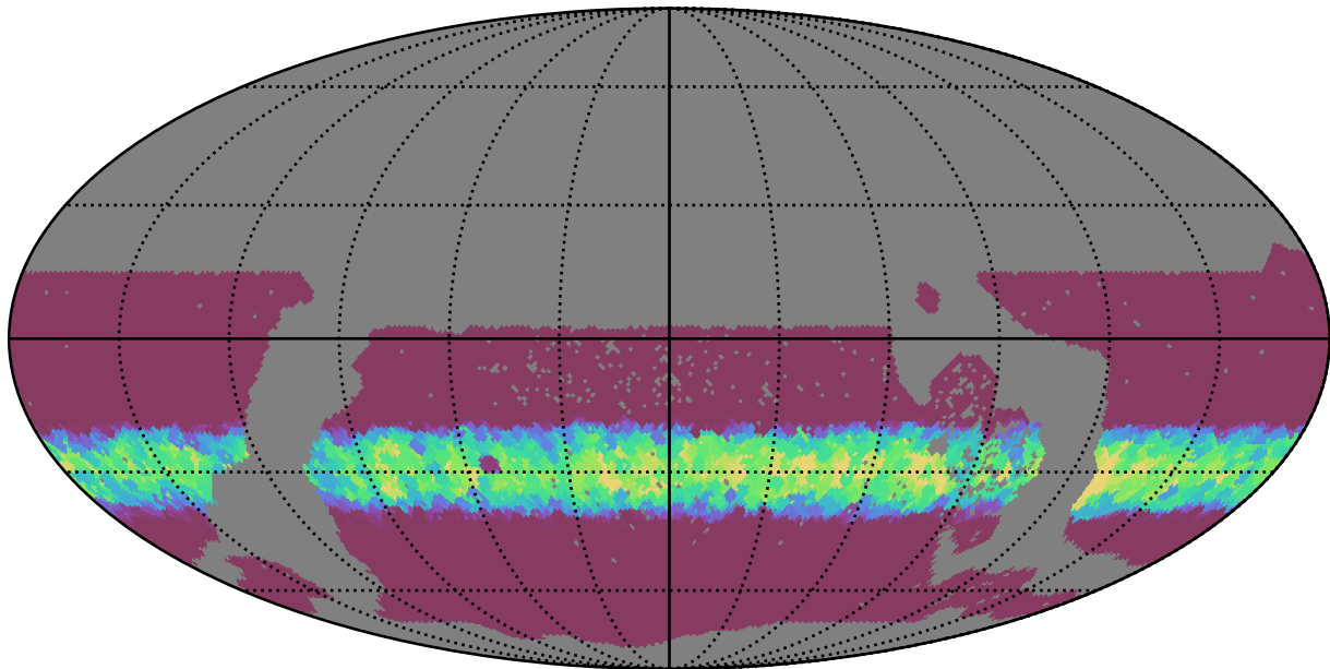
too_elab_r8_d3_giz_v3.4_10yrs WFD r band: Min normairmass
