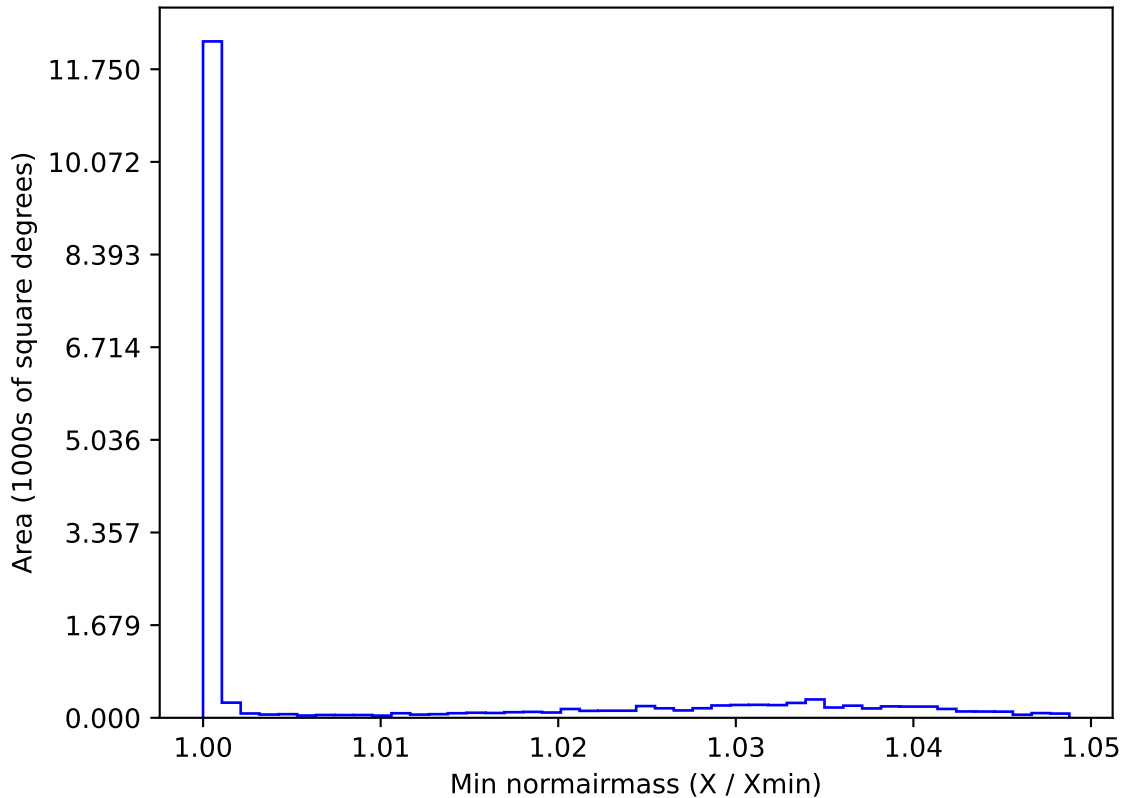
too_elab_r8_d3_giz_v3.4_10yrs WFD g band: Min normairmass
