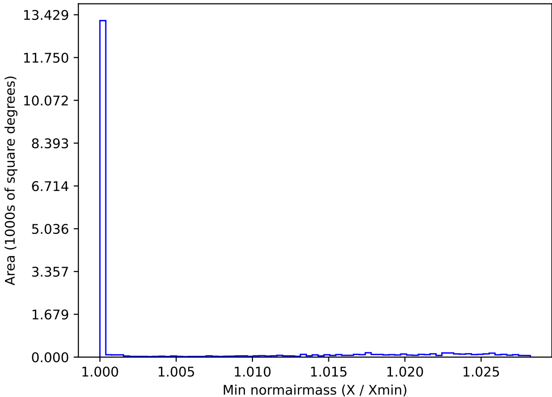
too_elab_r8_d3_giz_v3.4_10yrs WFD all bands: Min normairmass
