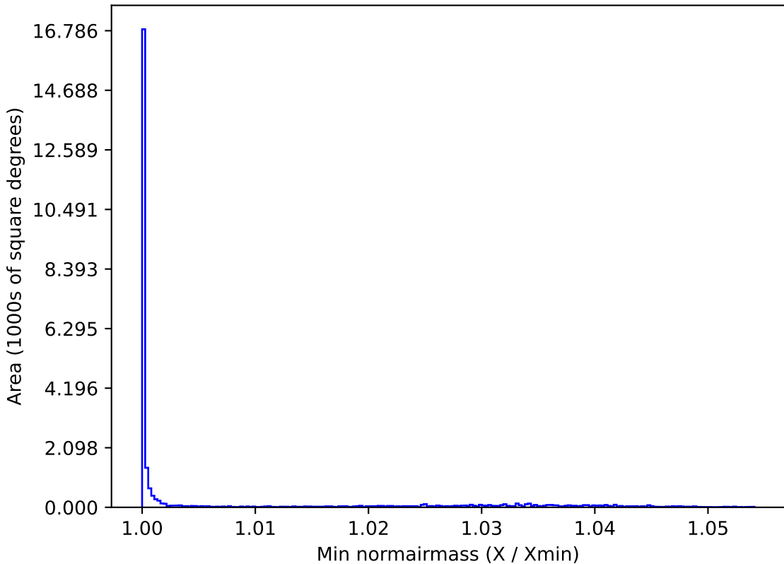
too_elab_r8_d3_giz_v3.4_10yrs All sky g band: Min normairmass
