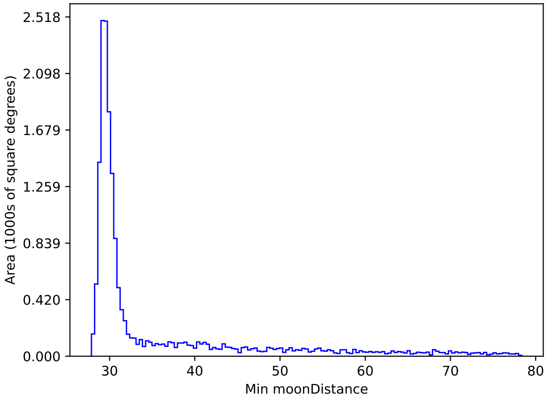
too_elab_r8_d3_giz_v3.4_10yrs WFD z band: Min moonDistance
