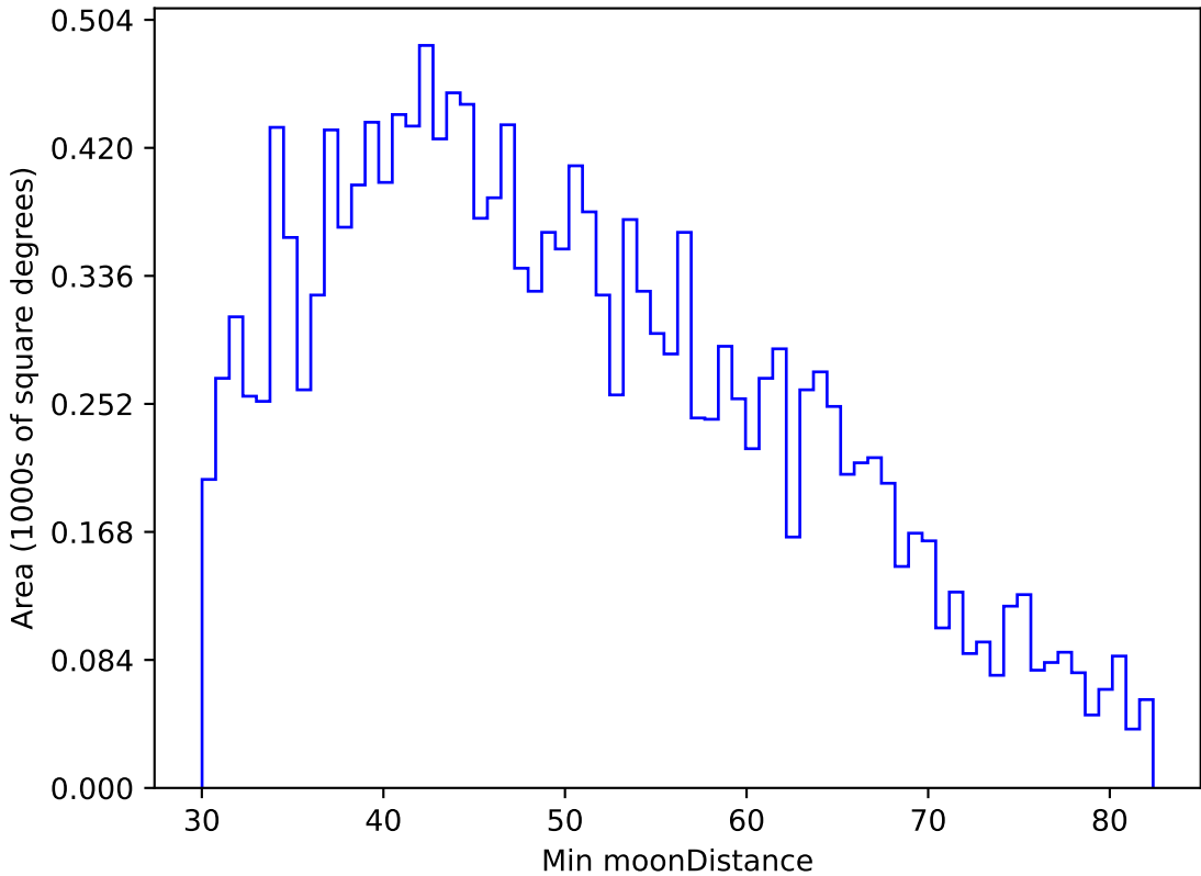
too_elab_r8_d3_giz_v3.4_10yrs WFD u band: Min moonDistance
