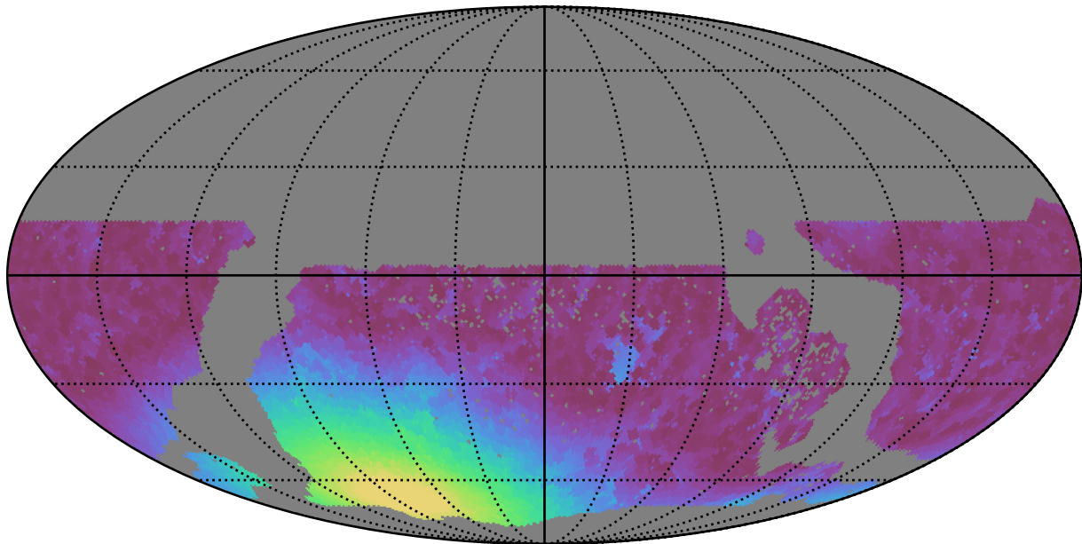
too_elab_r8_d3_giz_v3.4_10yrs WFD r band: Min moonDistance
