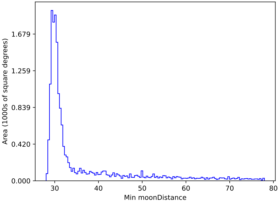
too_elab_r8_d3_giz_v3.4_10yrs WFD i band: Min moonDistance
