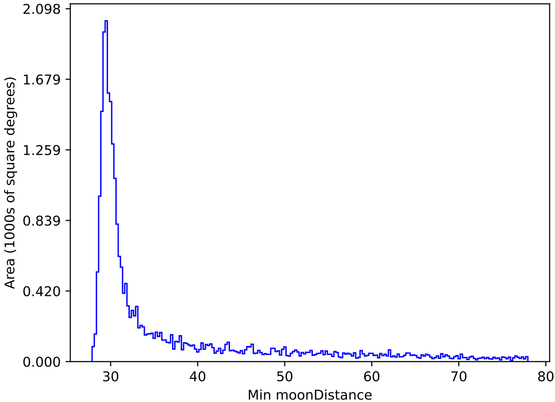
too_elab_r8_d3_giz_v3.4_10yrs All sky z band: Min moonDistance
