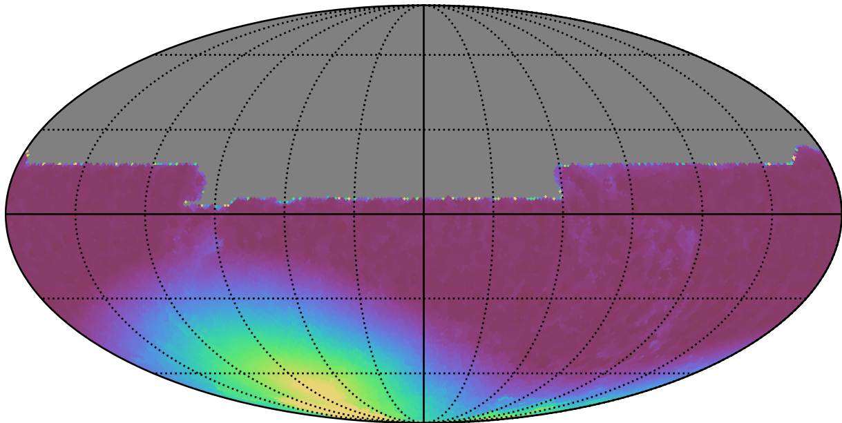
too_elab_r8_d3_giz_v3.4_10yrs All sky y band: Min moonDistance
