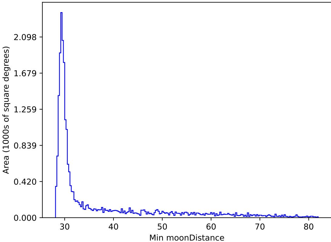
too_elab_r8_d3_giz_v3.4_10yrs All sky y band: Min moonDistance
