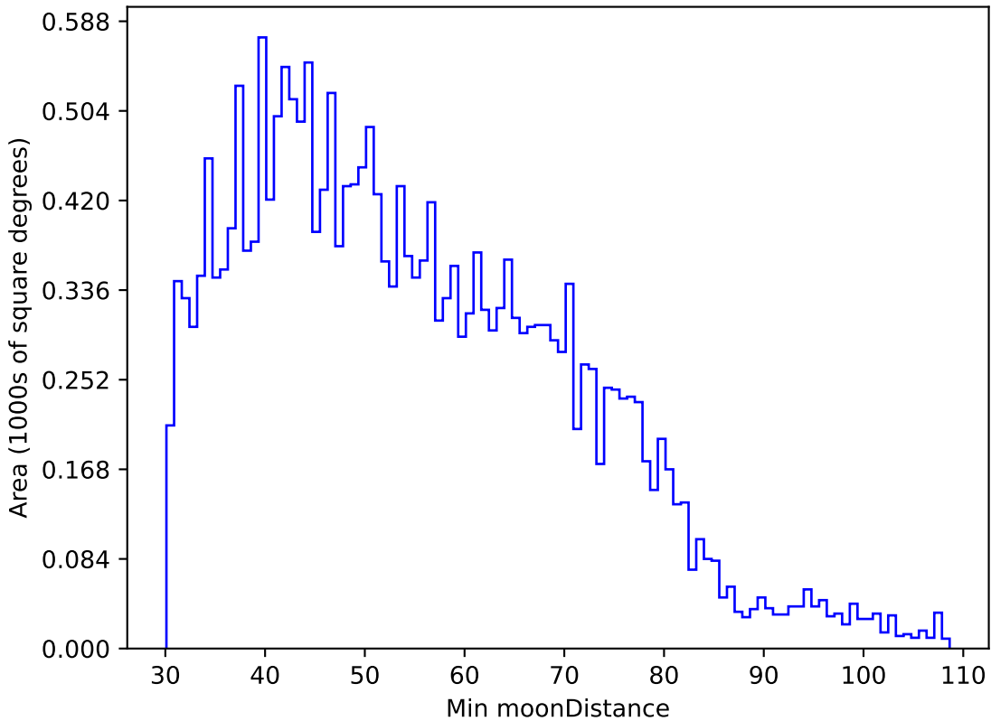
too_elab_r8_d3_giz_v3.4_10yrs All sky u band: Min moonDistance
