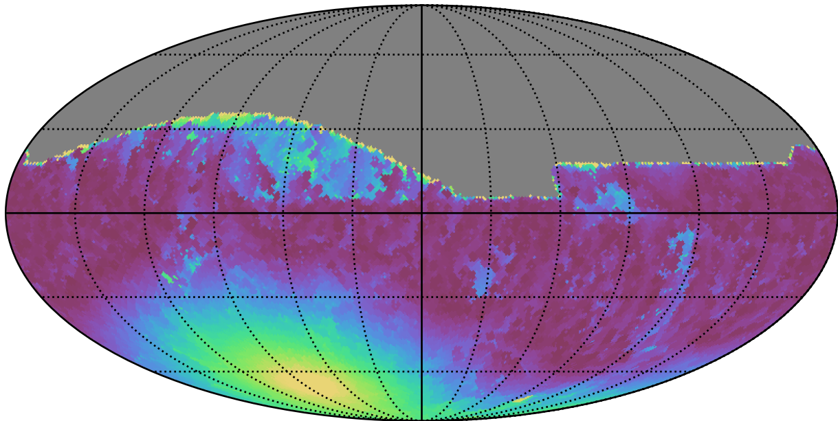
too_elab_r8_d3_giz_v3.4_10yrs All sky r band: Min moonDistance
