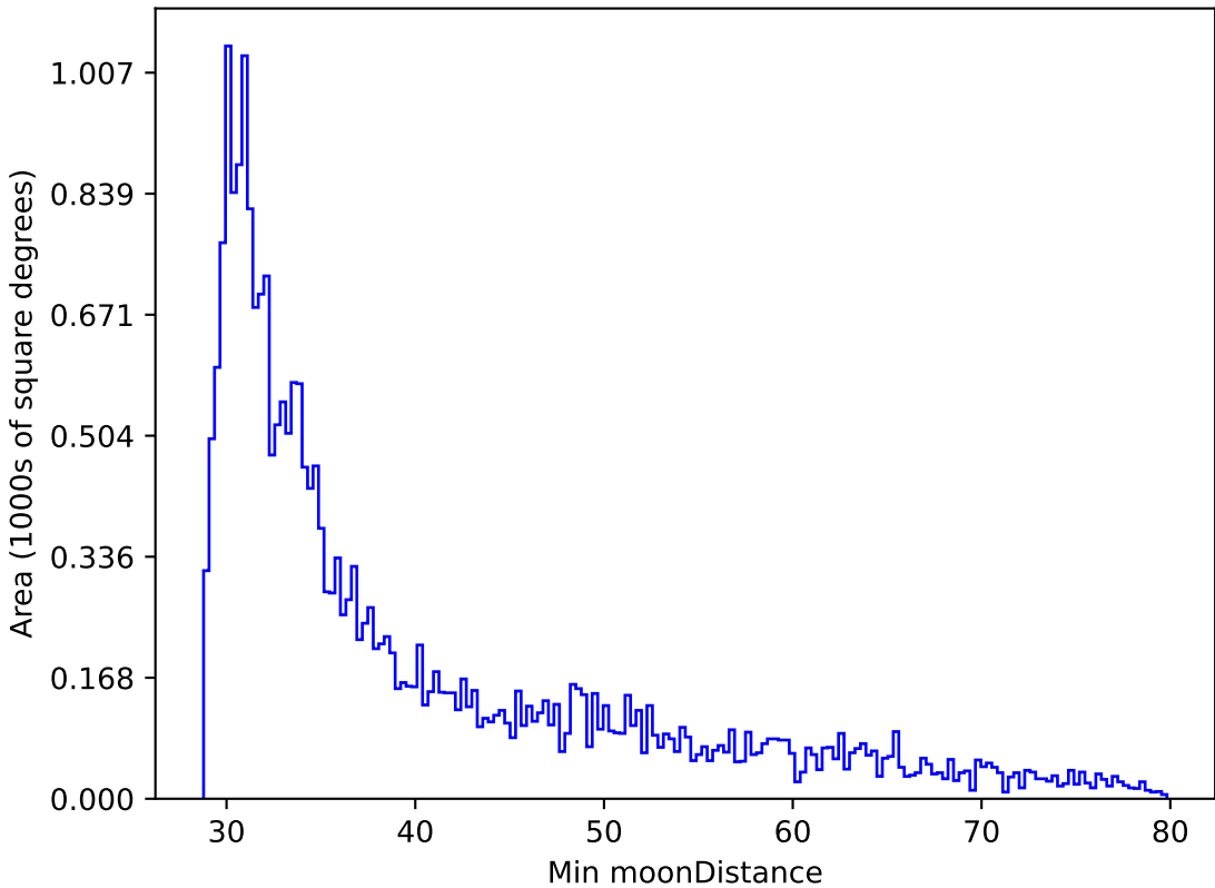
too_elab_r8_d3_giz_v3.4_10yrs All sky r band: Min moonDistance
