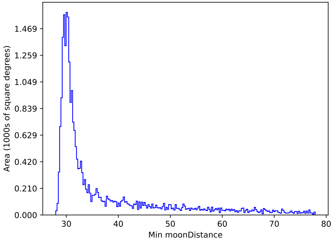
too_elab_r8_d3_giz_v3.4_10yrs All sky i band: Min moonDistance
